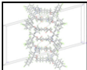
Fig. 2. The packing diagram of the title compound. Hydrogen bonds are shown as dashed lines.
