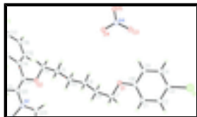
Fig. 1. The molecular structure of the title molecule, with the atom numbering scheme. Displacement ellipsoids are drawn at 30% probability levels.
